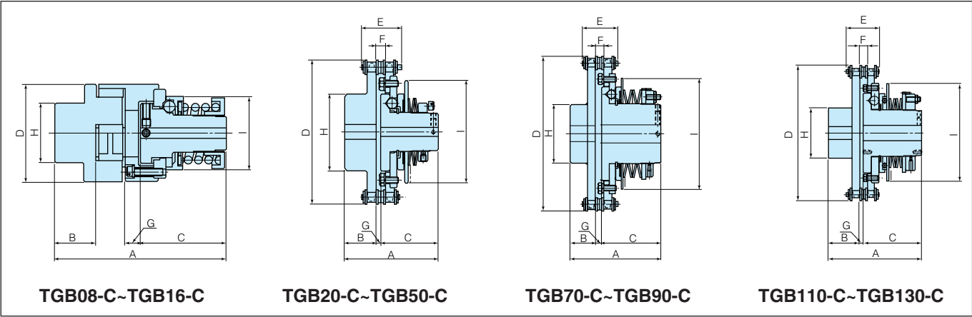
Dimensions of Torq Gard Coupling
