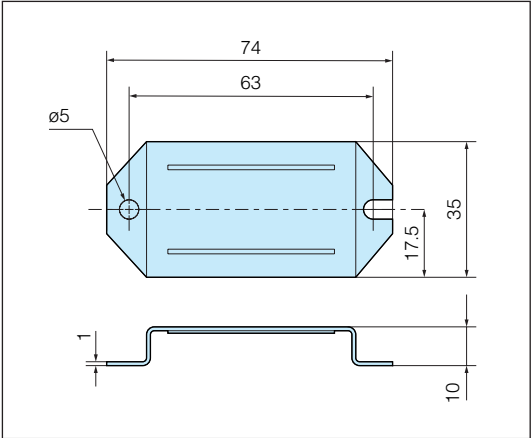
Mounting frame
